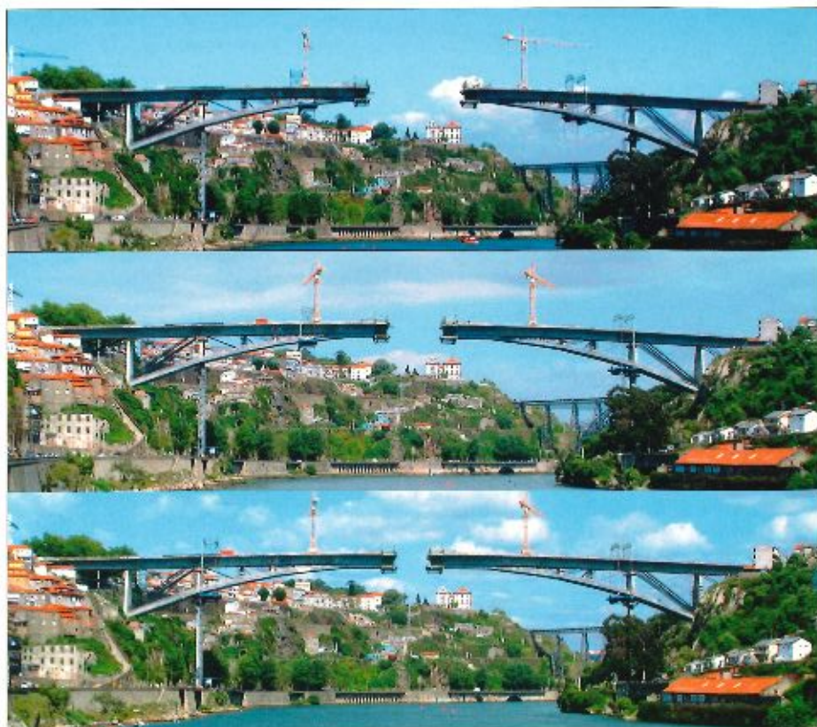
Fig. 3: Construction method
