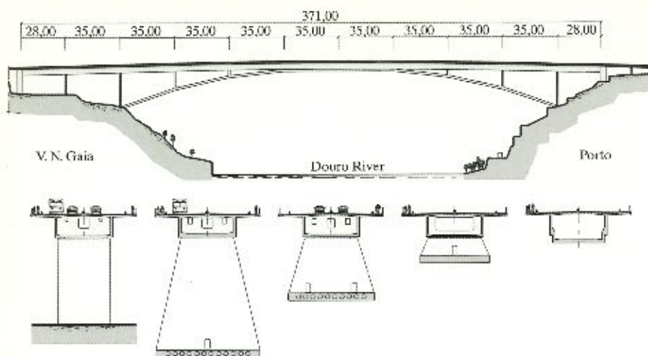
Fig. 2: Elevation and cross-sections of the bridge
