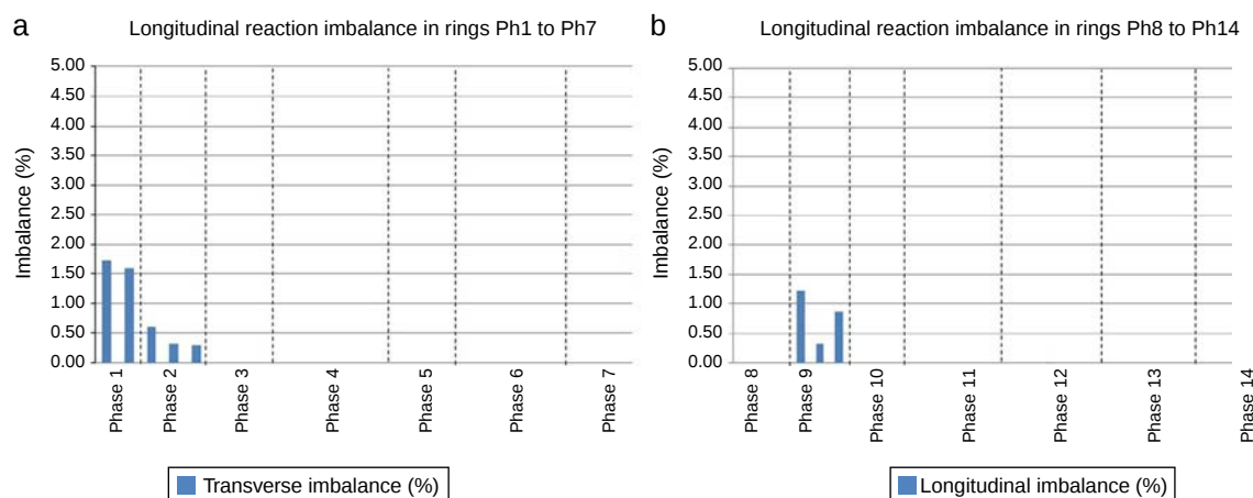
Figure 39. Longitudinal imbalance in the forward ring during concrete casting sub-phases in the 14 deck construction phases.
