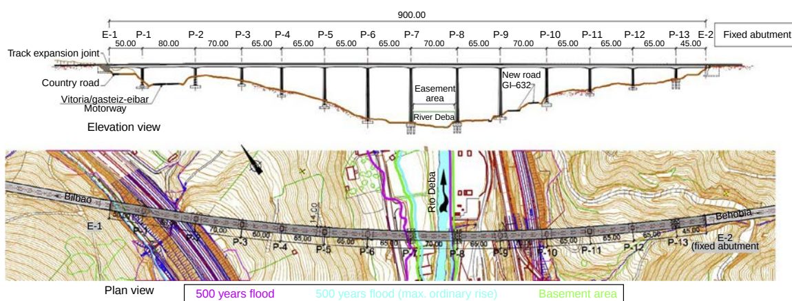
Figure 10. Elevation and plan views of the variable depth prestressed concrete deck ultimately built.
